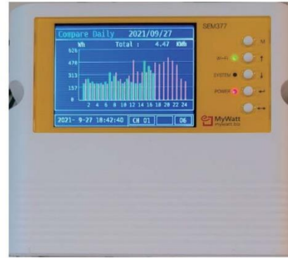
SEM377 Wall Mounting/Standing Smart Energy Manager
